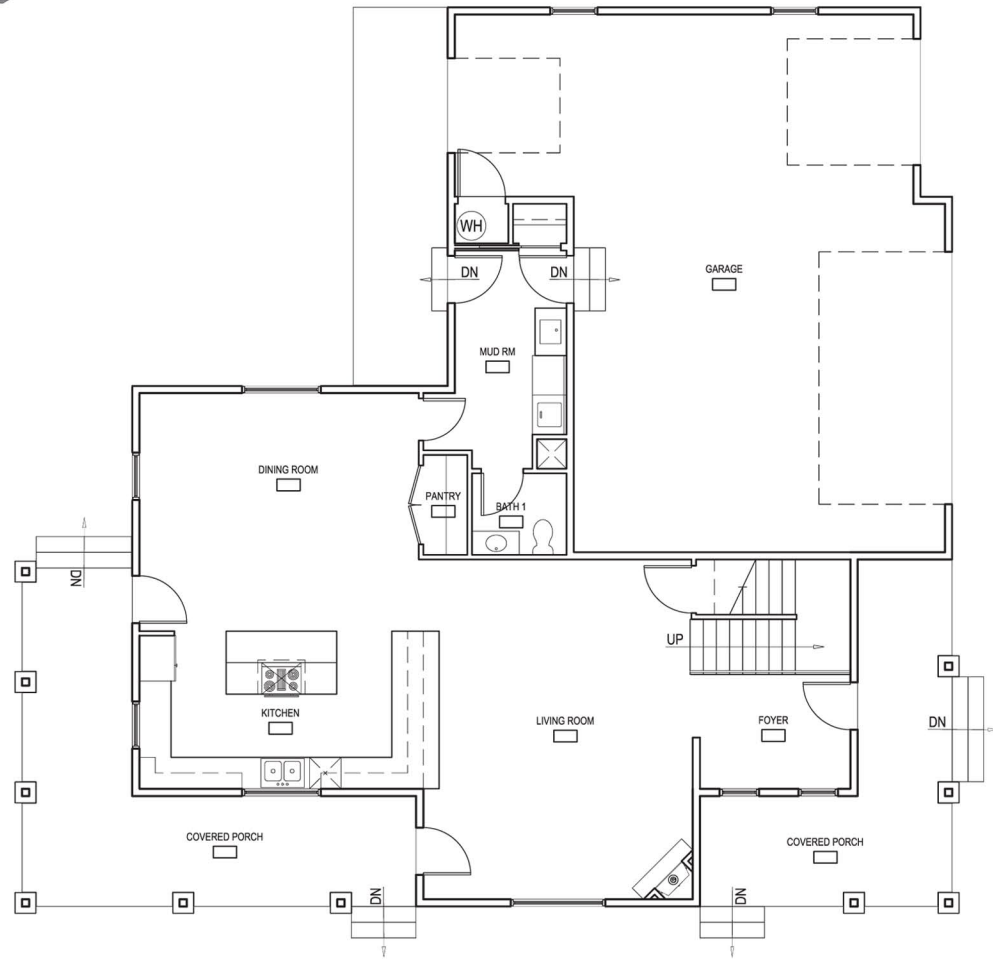
SECOND LEVEL PLAN N.T.S.
